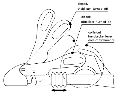
Fig. 5: Switching on stabiliser
