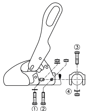
Croquis 3 : Raccordement
