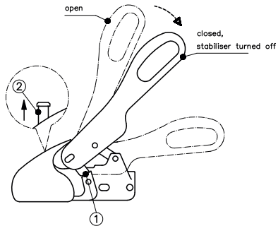
Fig. 4: Coupling
