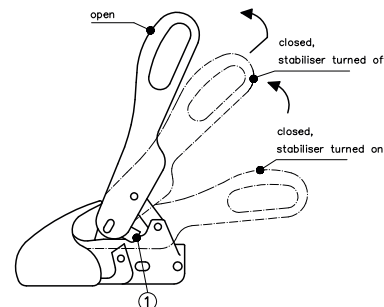
Fig. 6: Switching off stabiliser Disconnect
