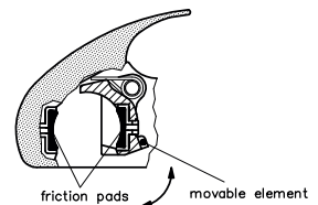
Fig. 9: Location of friction pads
